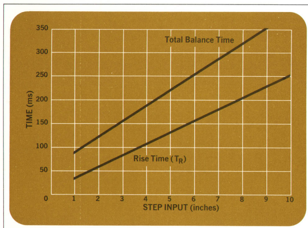
Fig. 3. Typical Y-axis response from a step input illustrates the relatively short time it takes for the pen to reach slewing speed.
